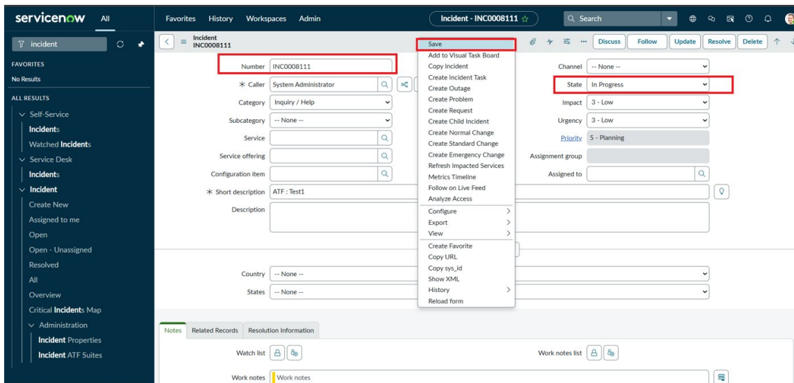
Figure 7: State changed on the Incident form (allowed).
