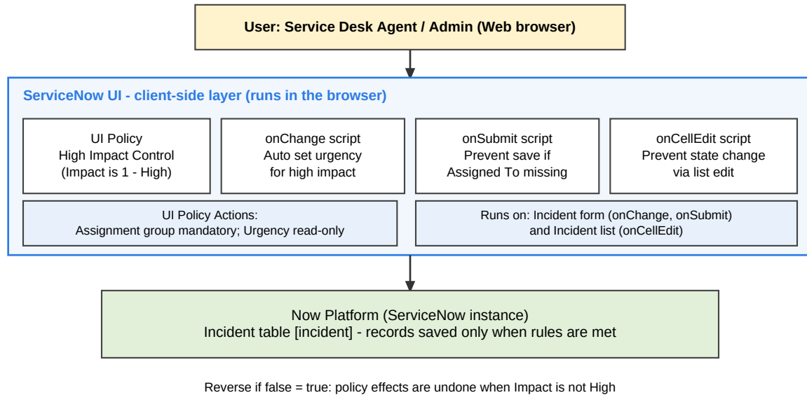
Figure 2: Client-side control layers on the Incident form and list.
