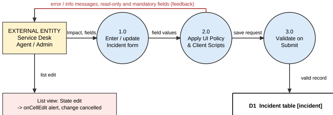
Figure 1: Data flow for the Incident form and list view.
